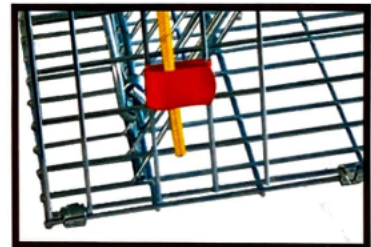
4. Make Sure U-Shape Support Bars (G) Are Completely Secured In Clip. Squeeze With Pliers Or Fingers To Prevent U-Shape Support Bars (G) From Popping Out.
