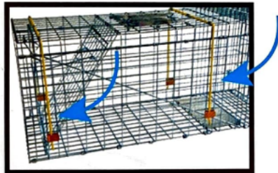
3. After Opening Cage, Make Sure Front Door (C) And Rear Door (B) Remain Inside The Trap, Lower U-Shape Support Bars (G) And Insert Ends Of Support Bars Into Support Clips (D).
